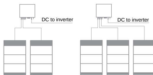
Connect 2 or 3 Battery Towers
