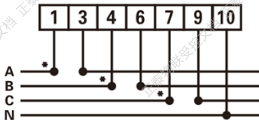
Figure12 Three phase four wire: direct connect
