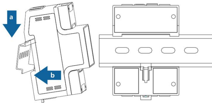
Figure11 Installation Diagram
