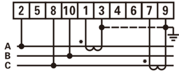
Figure15 Three phase three wire: via current transformer
