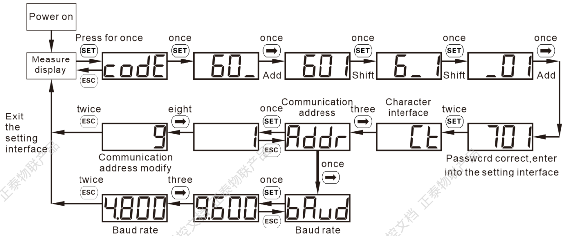
Figure5 Setting examples for communication address and Baud Rate
