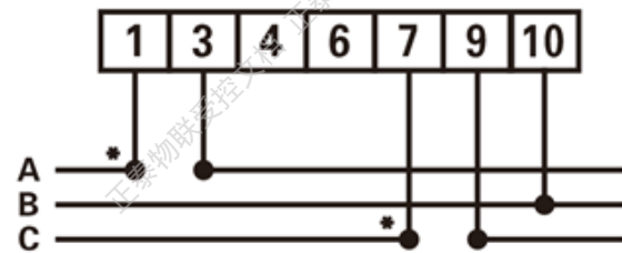
Figure13 Three phase three wire: direct connect
