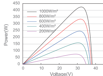
Power-Voltage Curve JAM54D40-425/GB
