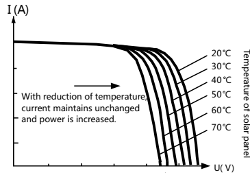
Fig.1-4 Relation Between Solar Battery Output Characteristics and Temperature
